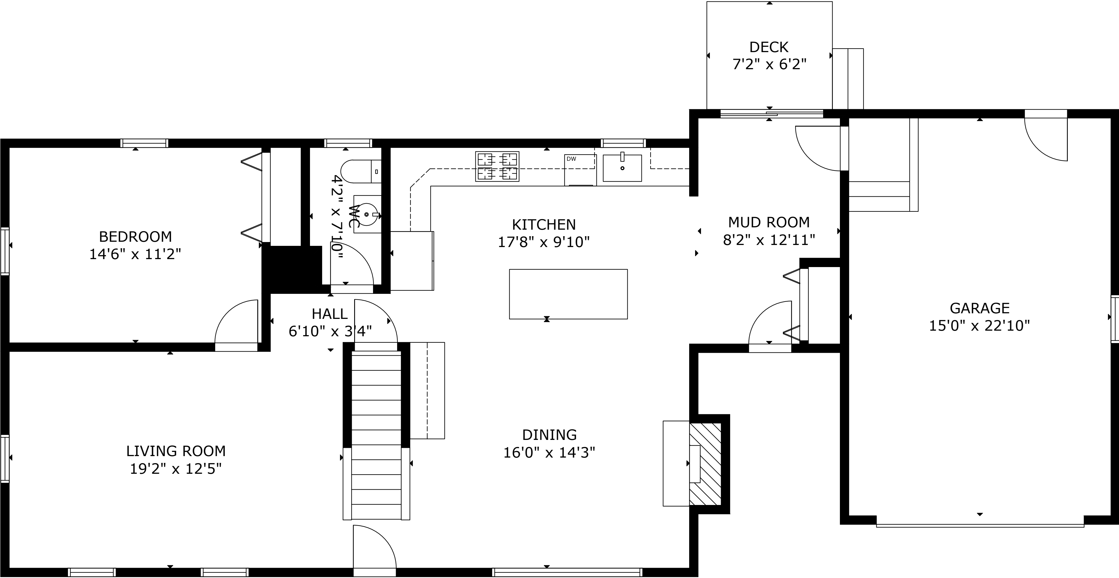
1ST FLOOR
